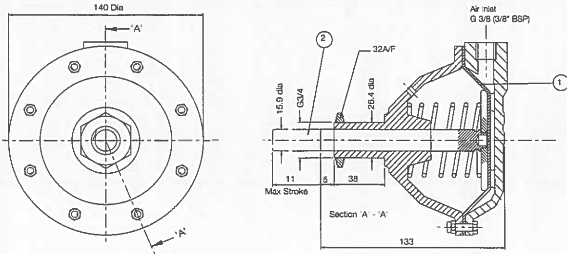
Thruster Part Number 7200276
